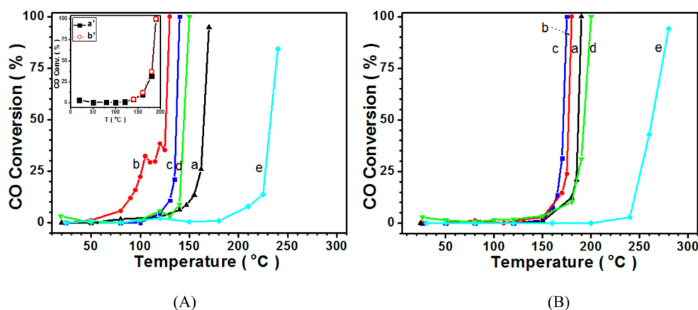
Figure 4. CO conversion over Pd 26 Ni 74 /C (black, a), Pd 56 Ni 44 /C (red, b), Pd 88 Ni 12 /C (blue, c), Pd/C (green, d), and Ni/C ((cyan, e) catalysts treated under H 2 (A) and O 2 (B). Inset in A: CO conversion activities for Pd 25 Ni 75 /C treated under H 2 , comparing data collected by increasing (black solid line, a') and decreasing (red dash line, b') the reaction temperature.
