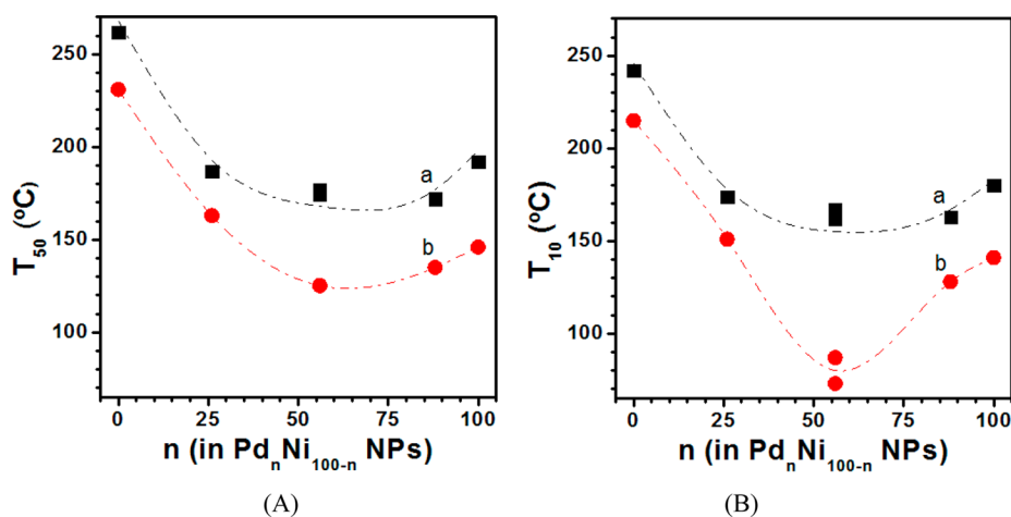
Figure 5. Plots of T_{50} (A) and T_{10} (B) vs n for Pd n Ni 100- n /C catalysts treated under O 2 at 450 °C for 30 min (a, black), and under H 2 at 300 °C for 30 min (b, red).
